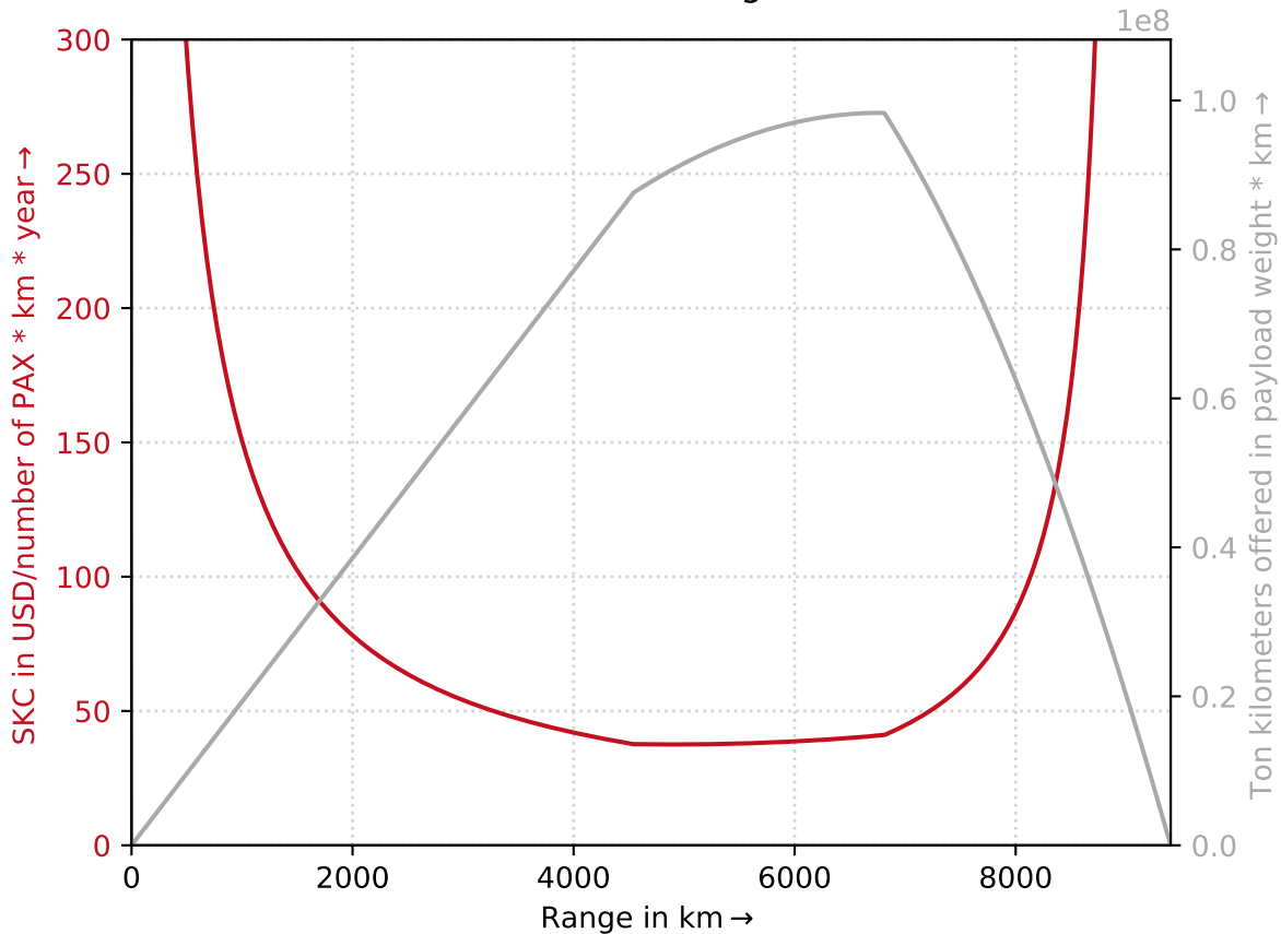
SKC and TKO for design mission
